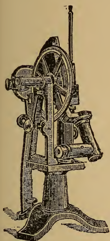
Fig. 61. AMAGAT-JEAN'S OLEO-REFRACTO- SCOPE FOR TESTING OILS AND BUTTER.
